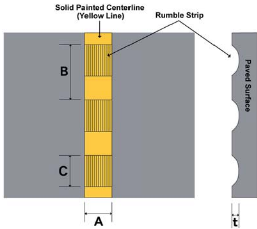
Figure 2-3: Rumble strip at a no-passing single-yellow centerline (specification)
