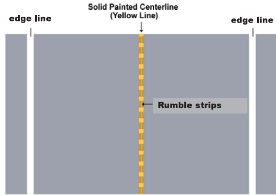
Figure 2-4: Rumble strip at a no-passing single-yellow centerline (installation location)
