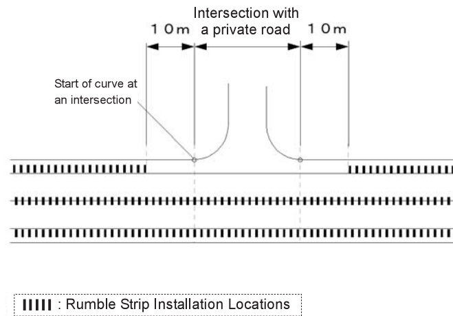
Figure 4-8: Example of installation at a junction with residential or other private roads
