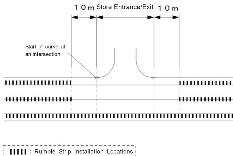
Figure 4-9: Example of installation on a commercial access road
