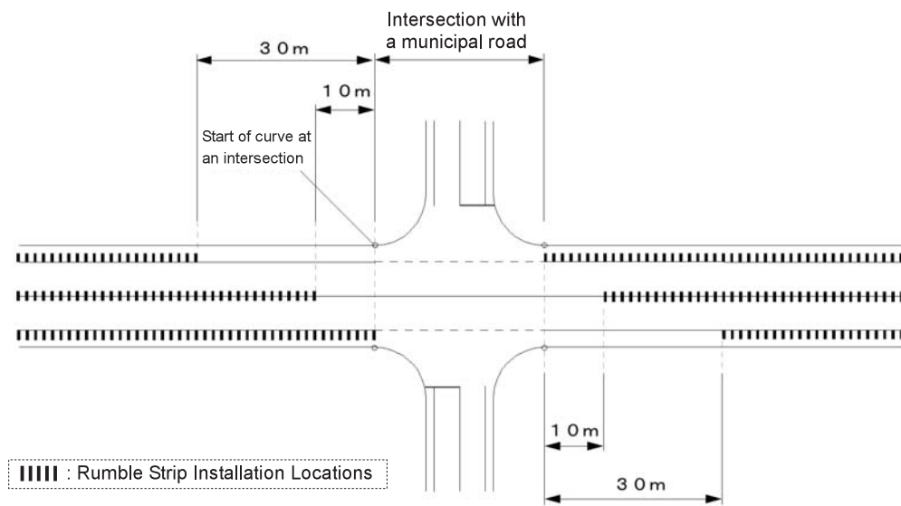
Figure 4-7: Example of installation at an intersection with a stop sign
