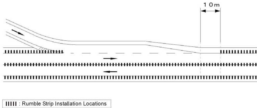
Figure 4-6: Example of installation at a merge section
