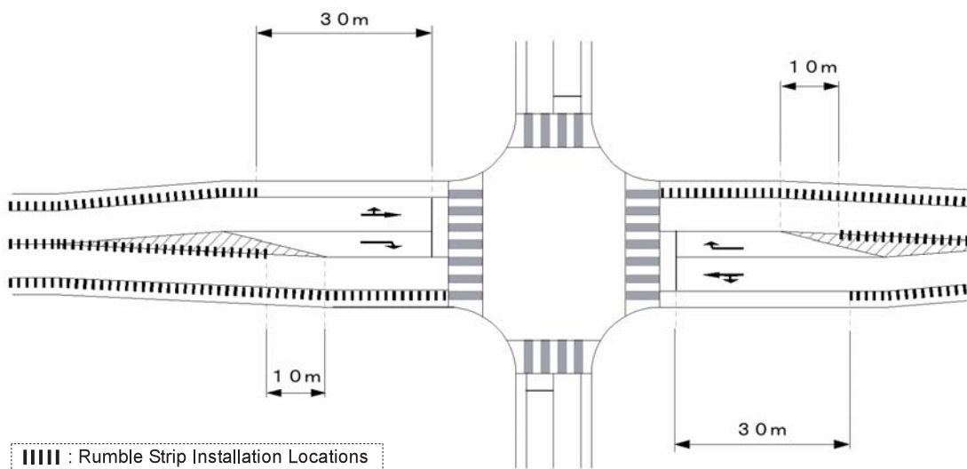
Figure 4-2: Installation example at an intersection with right-turn lane
