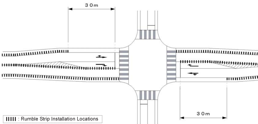
Figure 4-3: Installation example at an intersection with a right-turn lane
