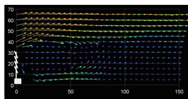
下部間隙閉塞率50% blockage rate of 50%
