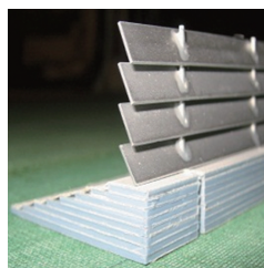
▲下部間隙閉塞率を変化させた風洞実験(閉塞率100%の例) Wind tunnel experiment with various rates of bottom gap blockage (blockage rate of 100%)
