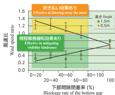
▲下部間隙閉塞率と風速比の関係 Relationship between the blockage rate of the bottom gap and the wind speed ratio
