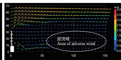
下部間隙閉塞率100% blockage rate of 100%
